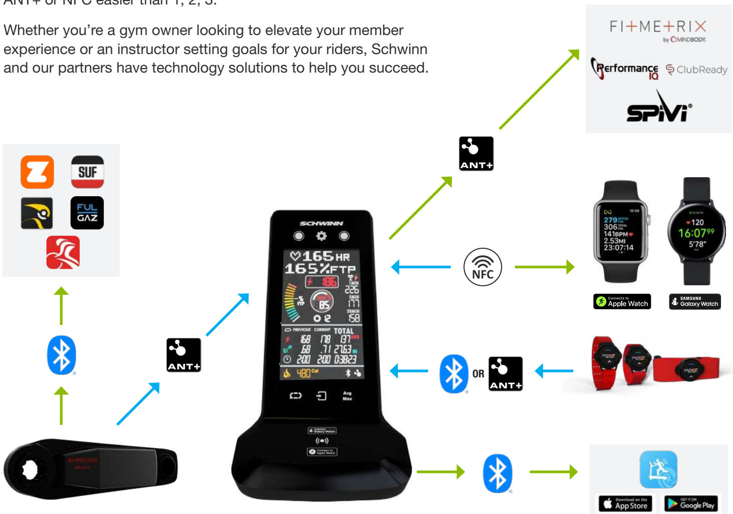
This diagram includes examples for each connection type but is not limited to the options shown.
